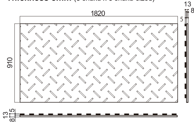
Thickness 8mm (3 shaku x 6 shaku-sized)
